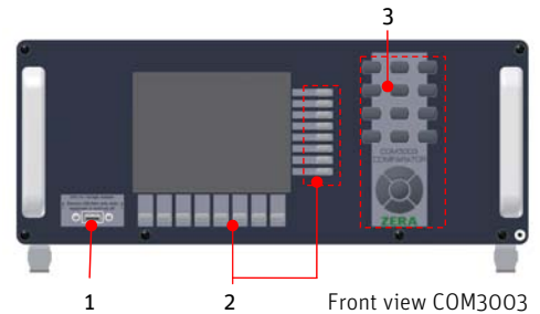
Front view COM3003 Three-phase Comparator
