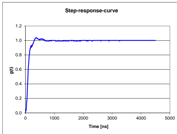
Example of a CS 700 step response
